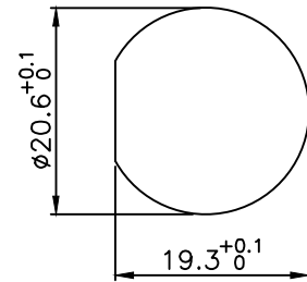
BOARD END HOLE OPENING SIZE
